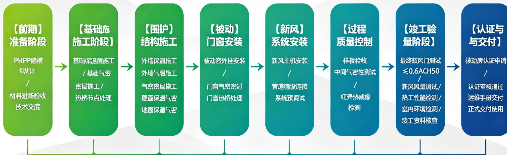
Passive House Installation & Delivery Standard Flowchart
